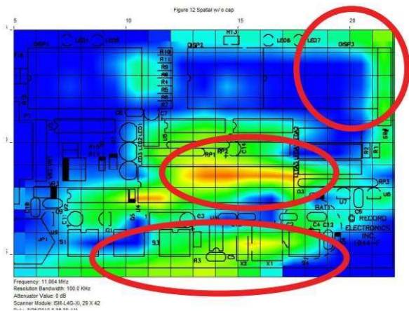
Taximeter PCB test with no capacitor – noise capacitor reduces circled in red.
