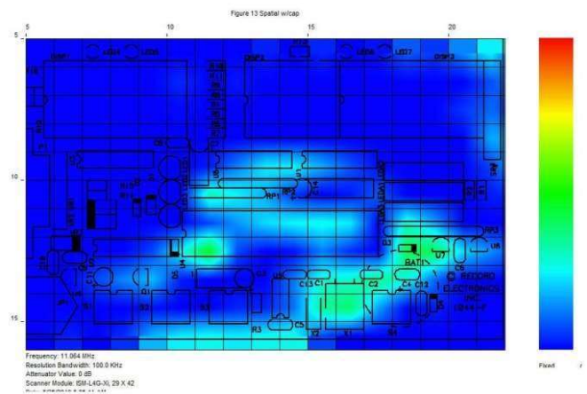
Taximeter PCB test with Noise by at least 8dBuV.
